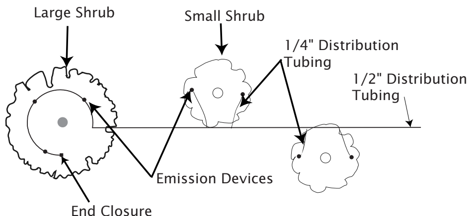
Figure 5-5: Emitter Placement
